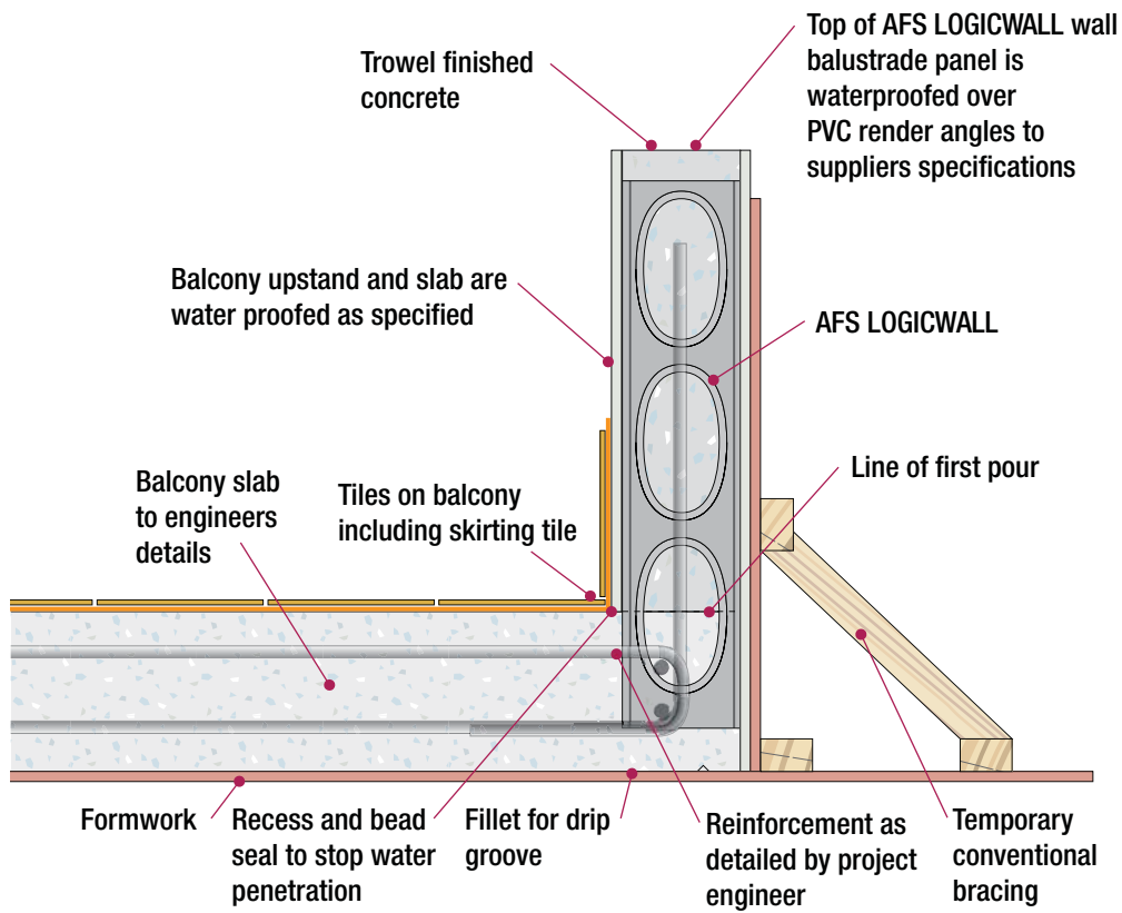
Fig I45: Balustrade Wall
