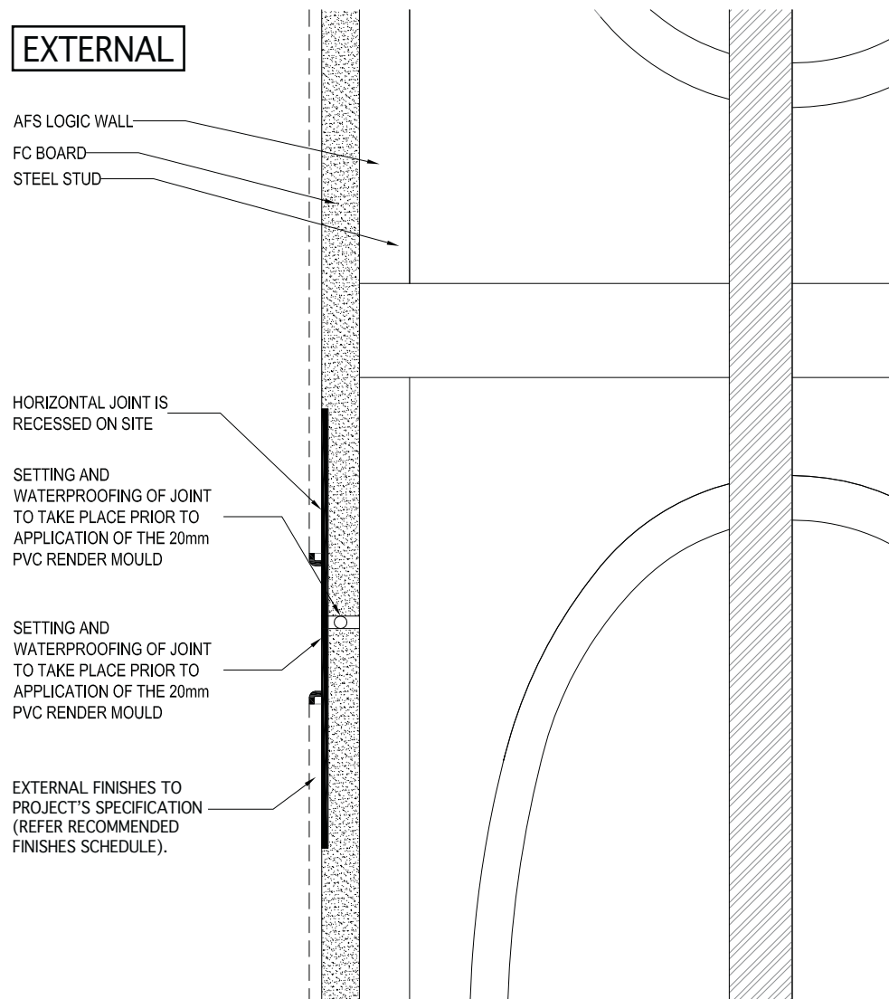
Fig I4: Horizontal 20mm Expressed Joint
